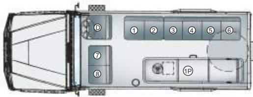
Seating Layout : D + 8 + 1P
